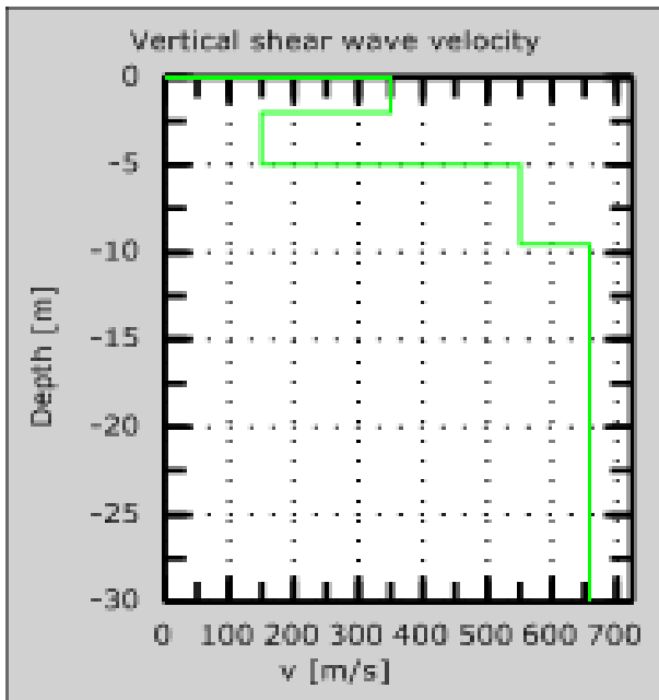
Figure 7: correct Vs profile from multi-modal apparent inversion.
