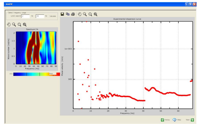
Figure 1: f-k spectrum and (v-f) exp dispersion curve.
