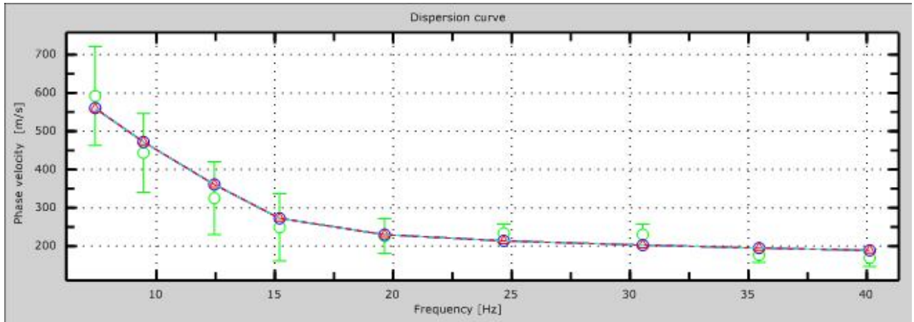
Figure 6: only fundamental mode inversion
