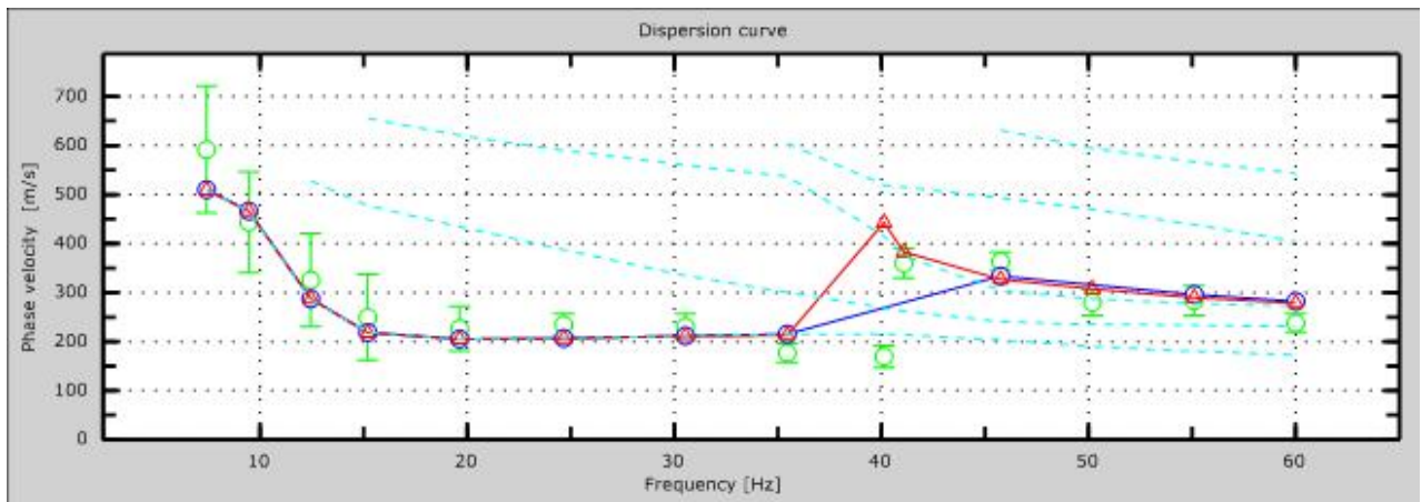
Figure 5: multi-modal apparent inversion.
